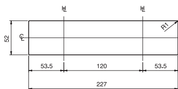
Panel Cutout T2MS253SF/T2MS253LF 3P
