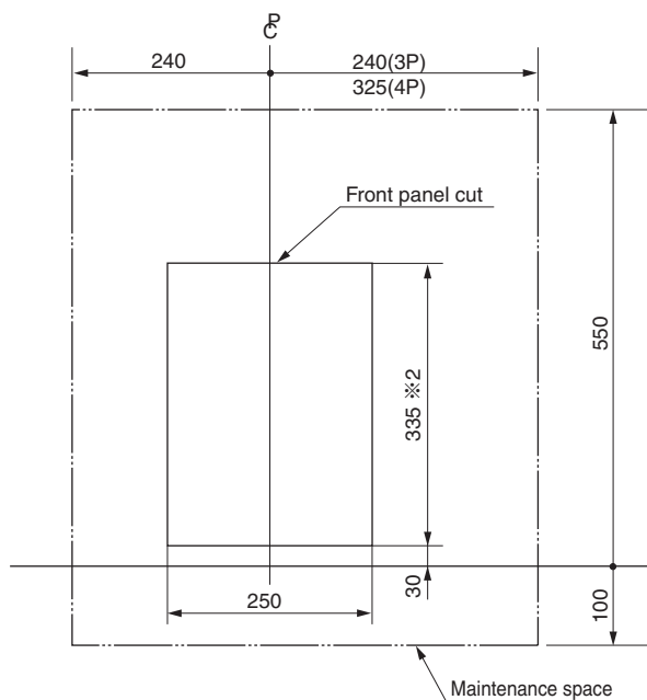
Panel cutout
