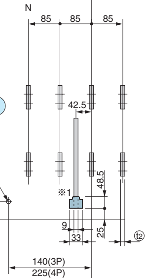
Vertical terminals
