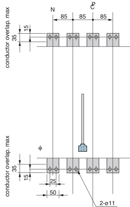
Front connections
