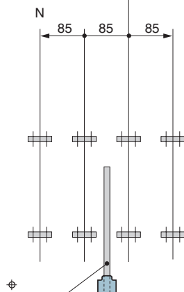
Horizontal terminals
