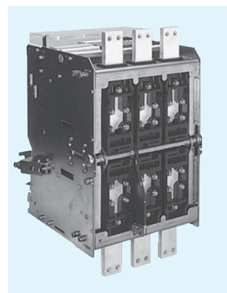
▲Front connections
