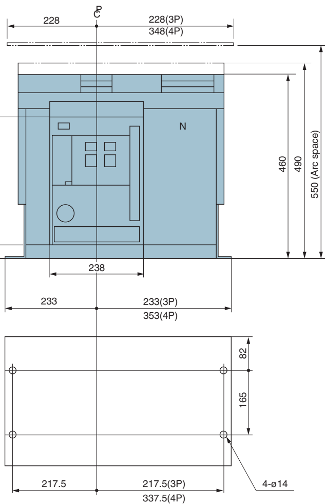
Mounting holes
