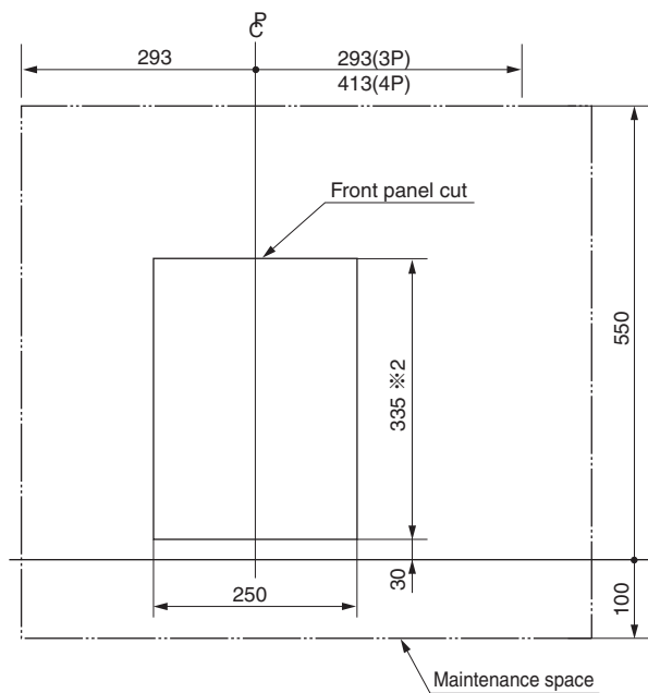
Panel cutout
